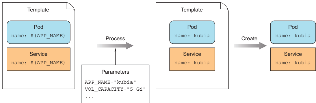
Figure 18.8 OpenShift templates
