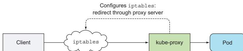
Figure 11.9 The userspace proxy mode
